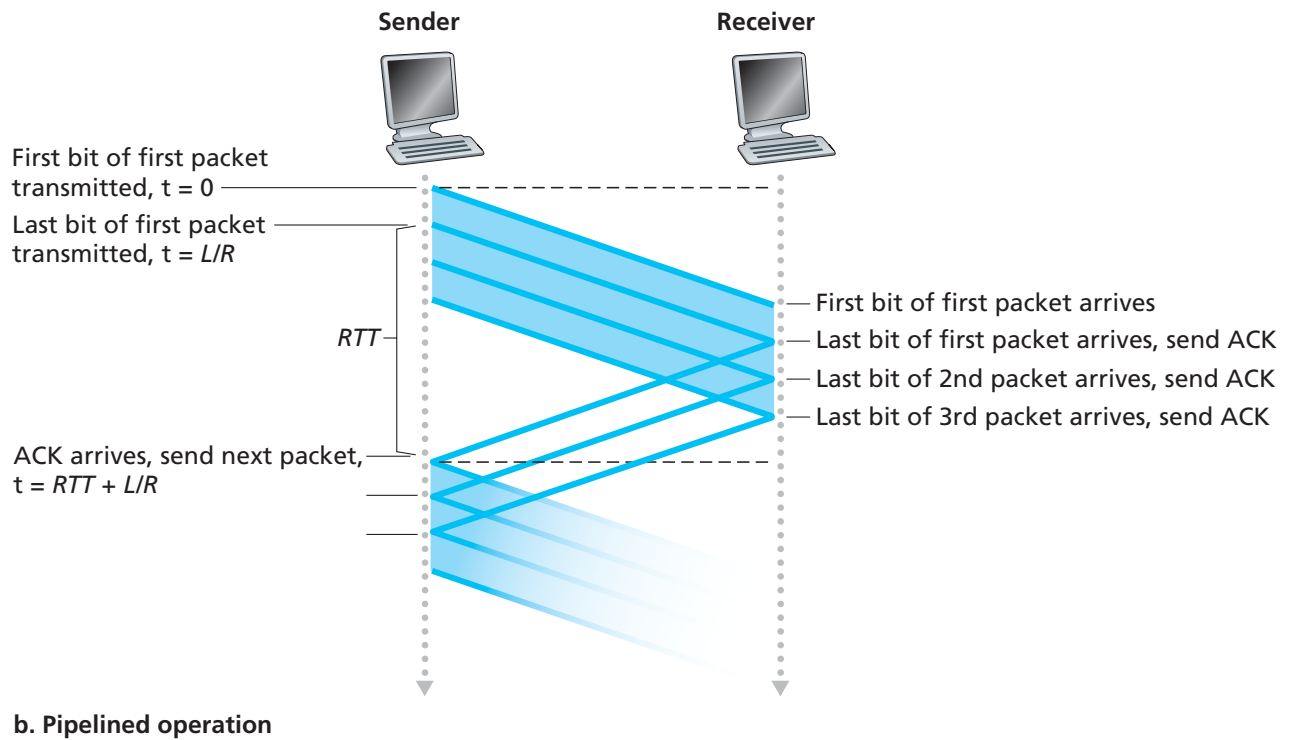
Figure 3.18 ♦ Stop-and-wait and pipelined sending
