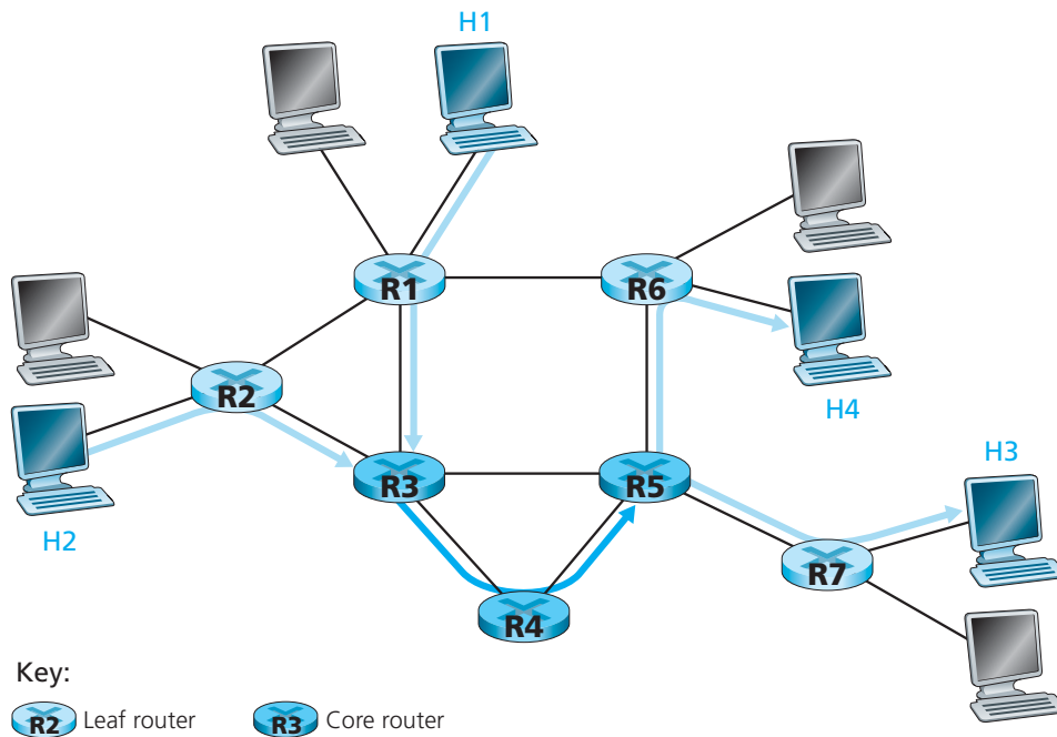
Figure 7.25 ♦ A simple Diffserv network example
