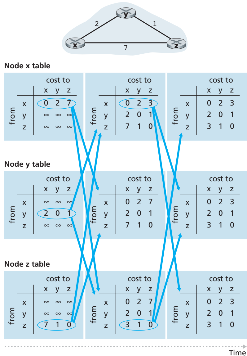
Figure 4.30 ♦ Distance-vector (DV) algorithm
