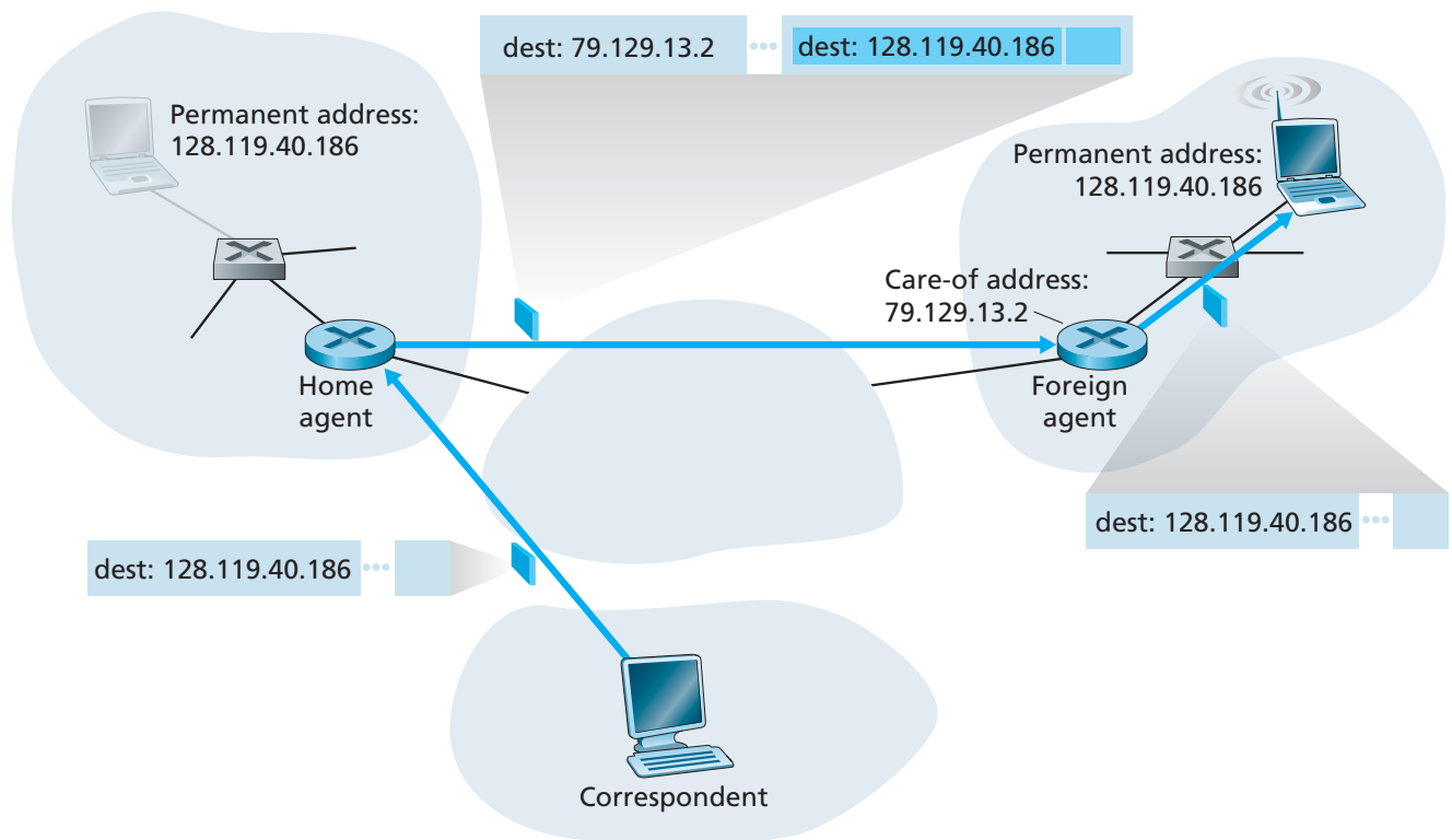
Figure 6.24 ♦ Encapsulation and decapsulation
