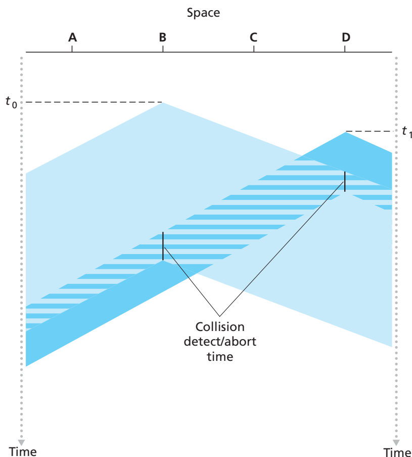
Figure 5.13 ♦ CSMA with collision detection
