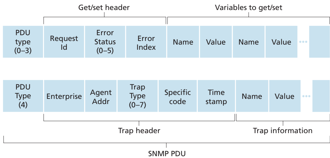
Figure 9.4 ♦ SNMP PDU format
