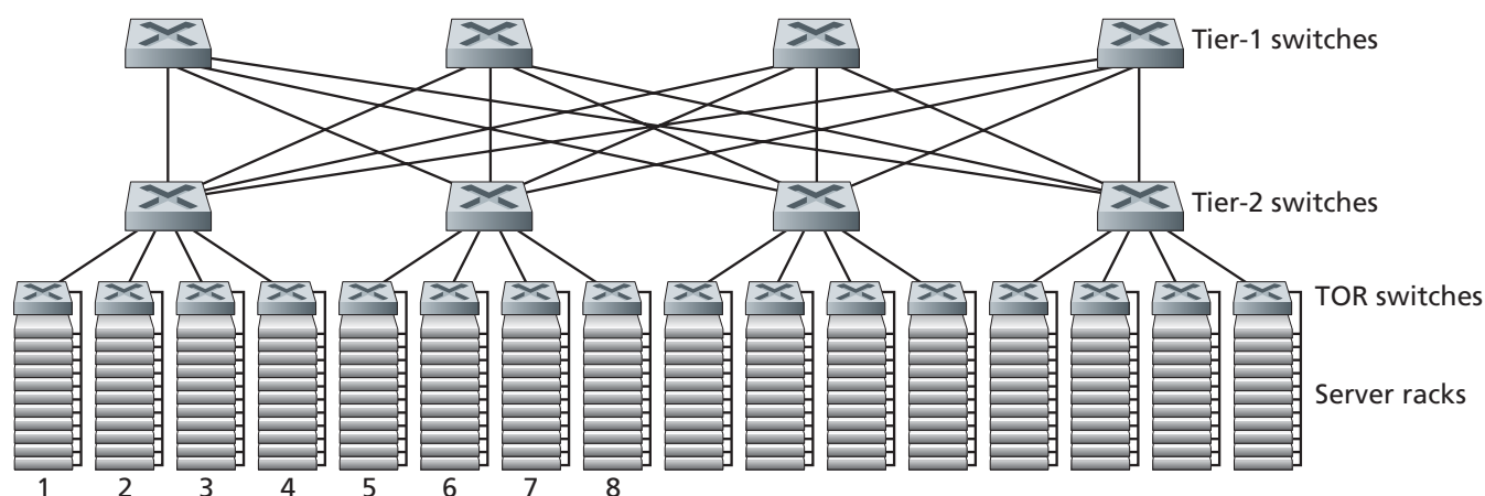
Figure 5.31 ♦ Highly-interconnected data network topology
