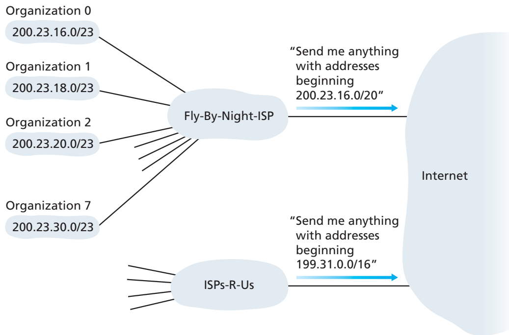
Figure 4.18 ♦ Hierarchical addressing and route aggregation
