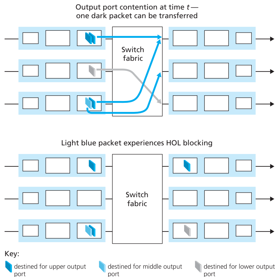
Figure 4.11 ♦ HOL blocking at an input queued switch
