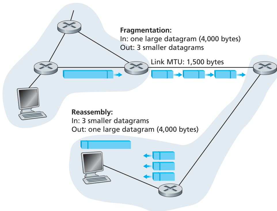
Figure 4.14 ♦ IP fragmentation and reassembly
