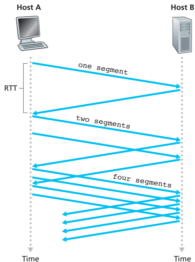
Figure 3.51 ♦ TCP slow start
