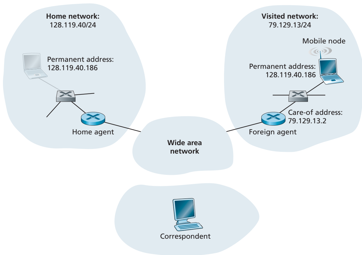
Figure 6.22 ♦ Initial elements of a mobile network architecture
