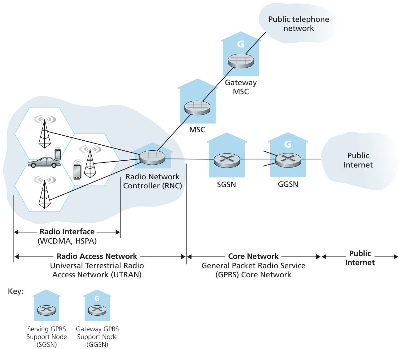
Figure 6.19 ♦ 3G system architecture
