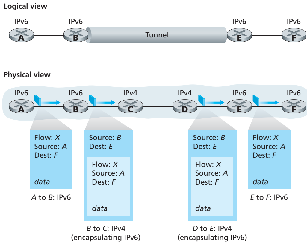
Figure 4.26 ♦ Tunneling
