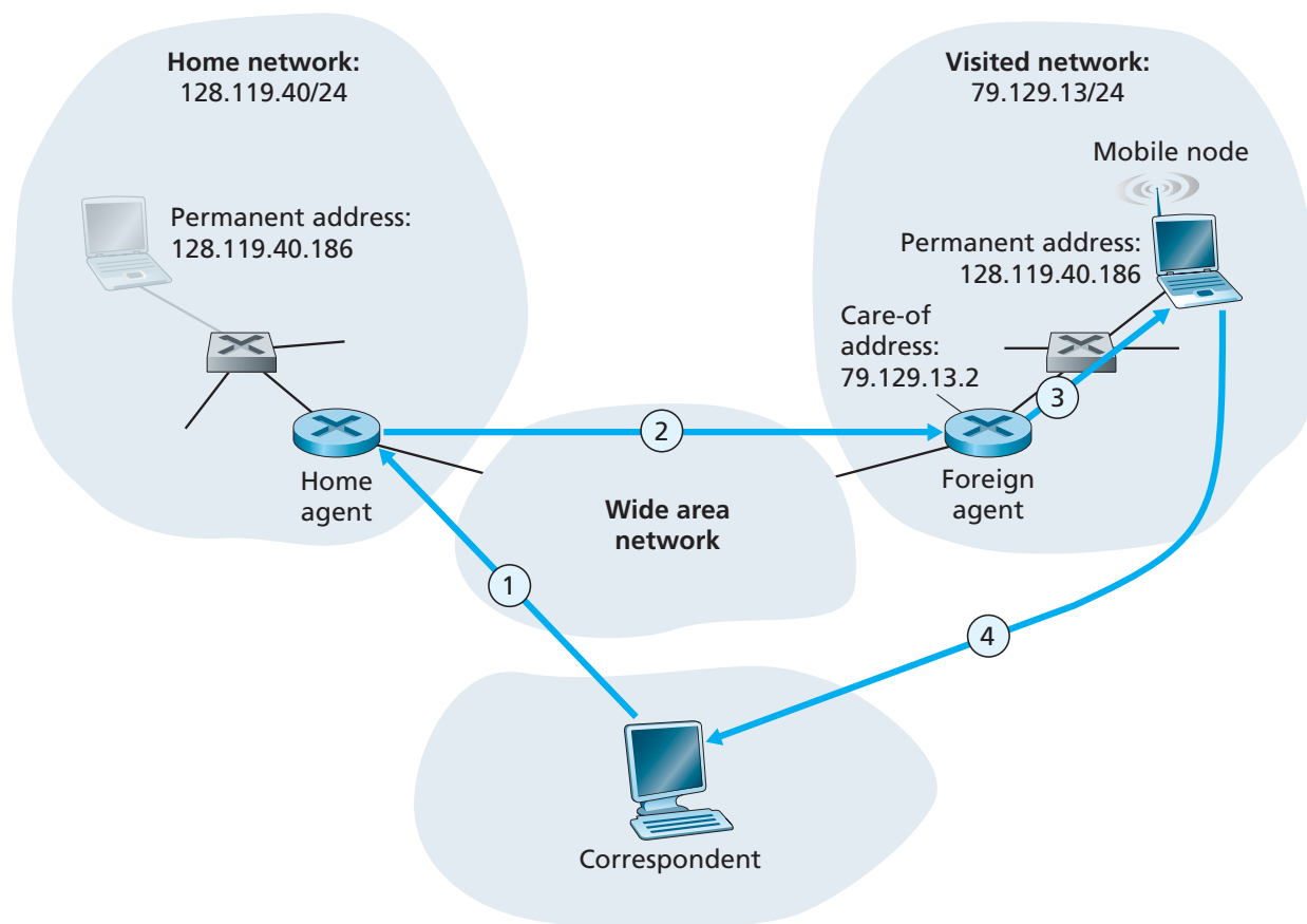
Figure 6.23 ♦ Indirect routing to a mobile node
