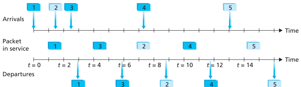
Figure 7.20 ♦ Operation of the priority queue
