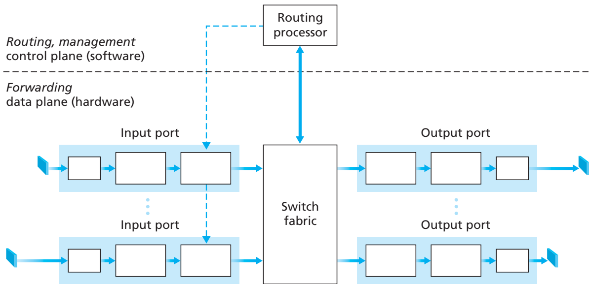
Figure 4.6 ♦ Router architecture
