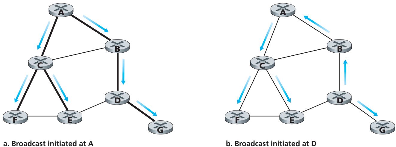
Figure 4.45 ♦ Broadcast along a spanning tree
