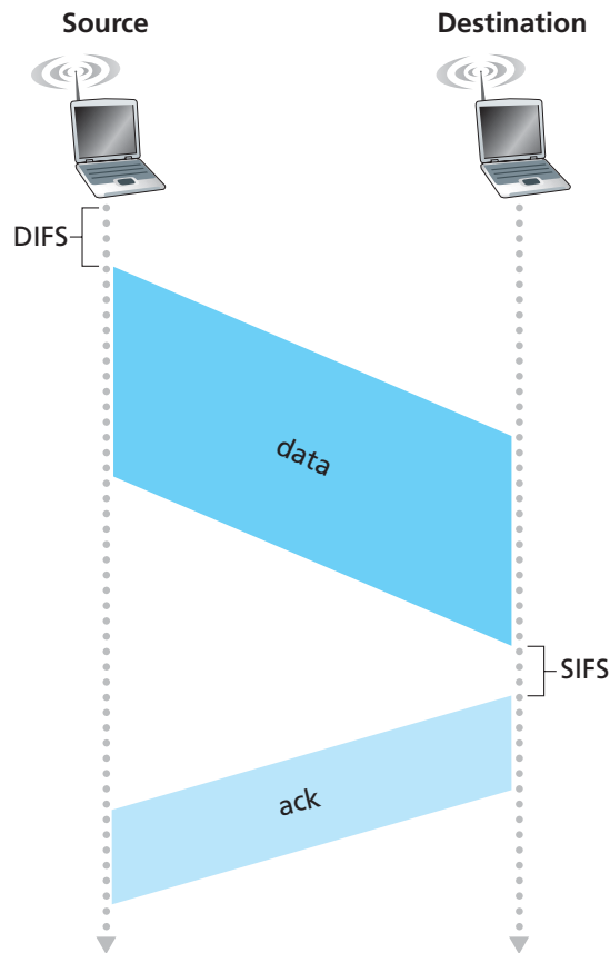
Figure 6.10 ♦ 802.11 uses link-layer acknowledgments
