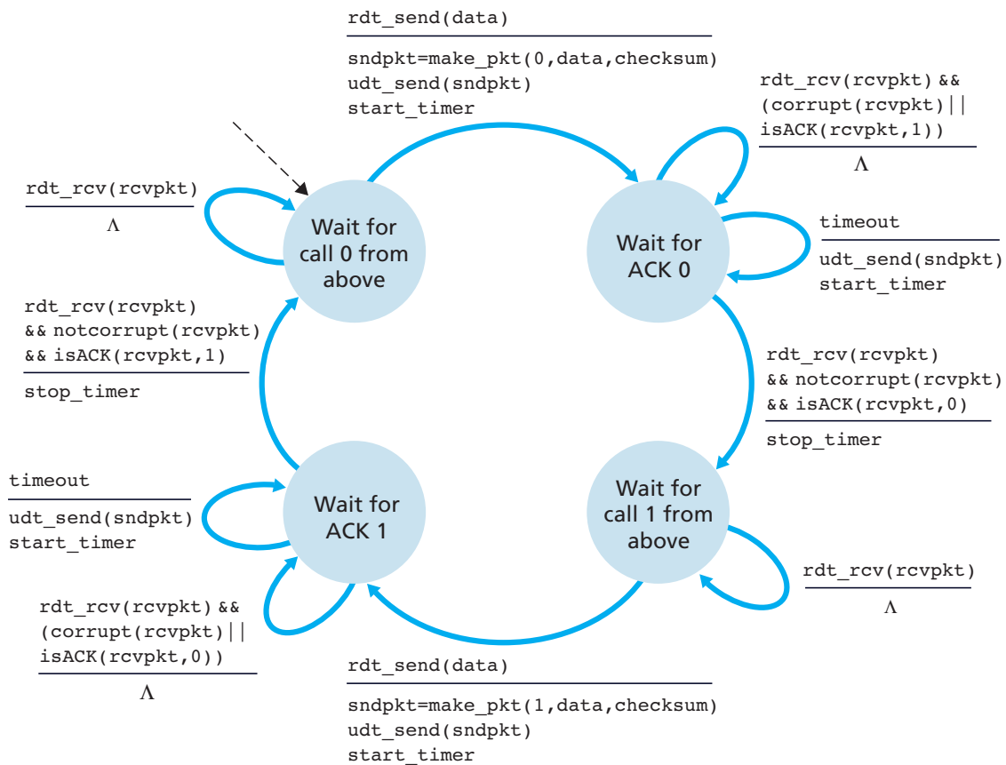
Figure 3.15 ♦ rdt3.0 sender
