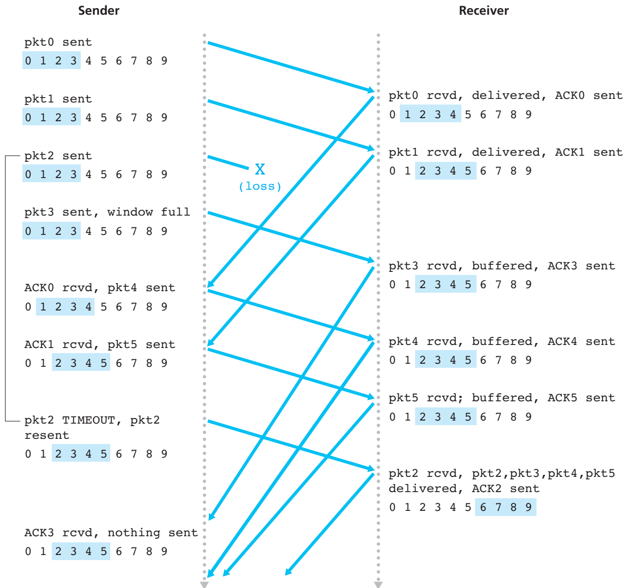
Figure 3.26 ♦ SR operation
