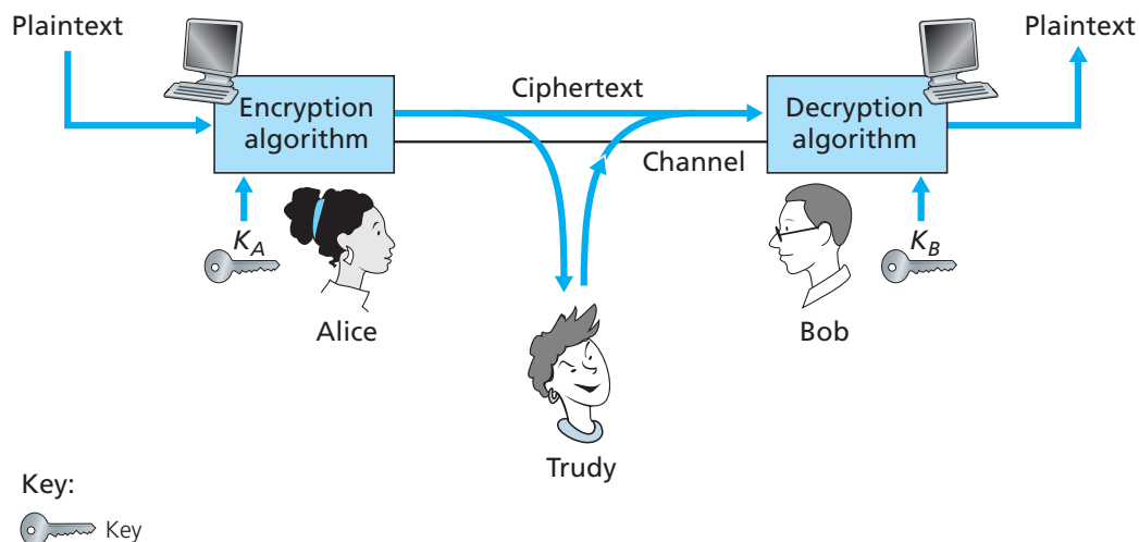
Figure 8.2 ♦ Cryptographic components
