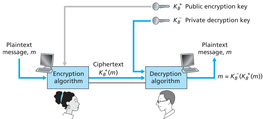
Figure 8.6 ♦ Public key cryptography
