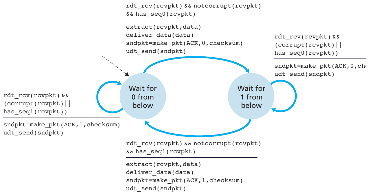
Figure 3.14 ♦ rdt2.2 receiver
