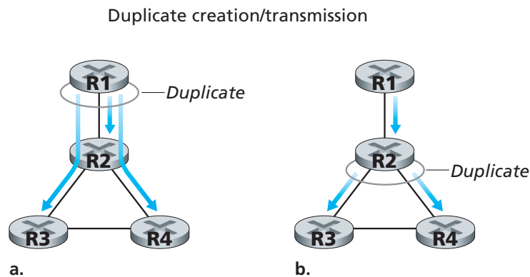
Figure 4.43 ♦ Source-duplication versus in-network duplication
