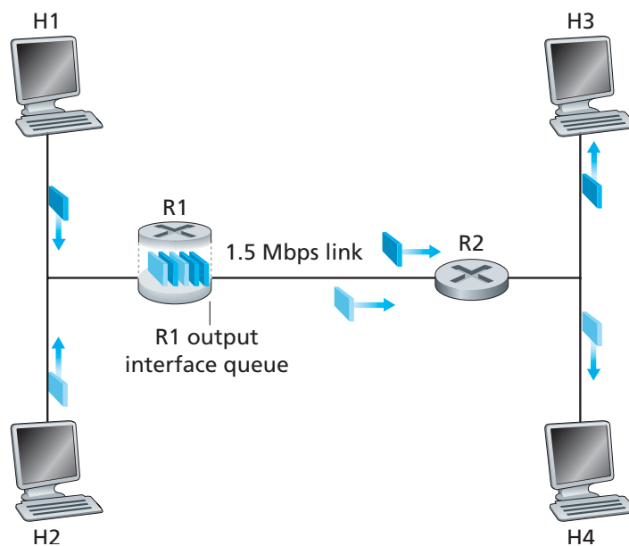
Figure 7.17 ♦ FIFO queuing abstraction
