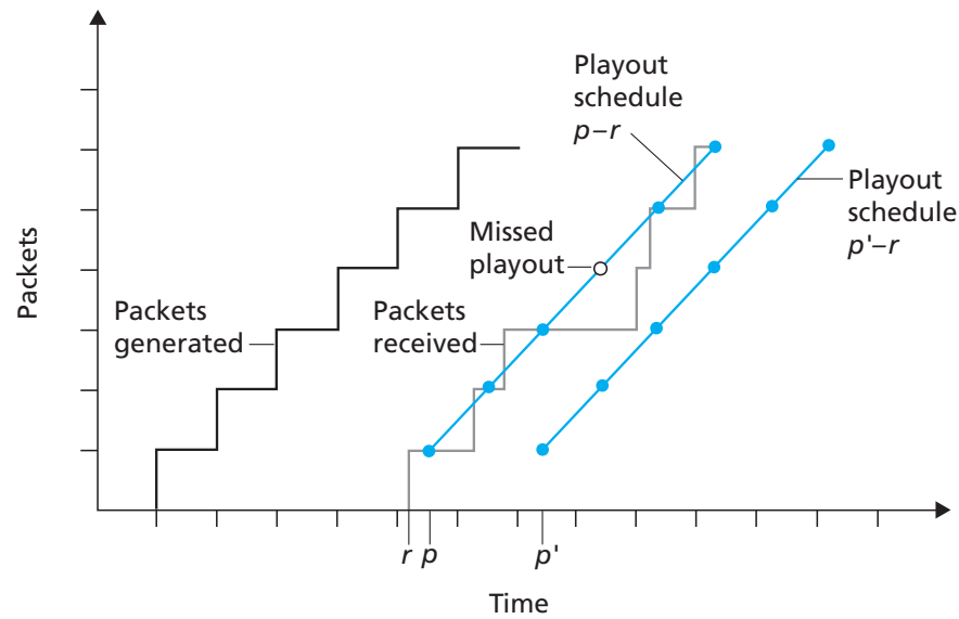
Figure 7.7 ♦ Packet loss for different fixed playout delays
