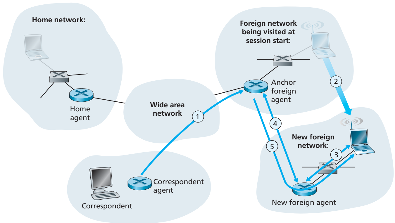
Figure 6.26 ♦ Mobile transfer between networks with direct routing
