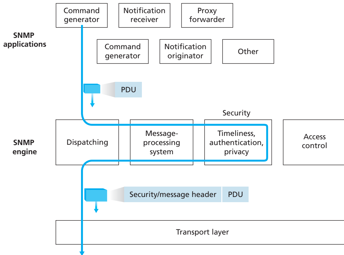
Figure 9.5 ♦ SNMPv3 engine and applications
