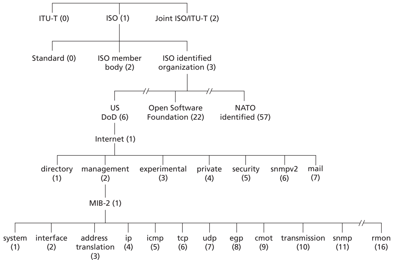
Figure 9.3 ♦ ASN.1 object identifier tree
