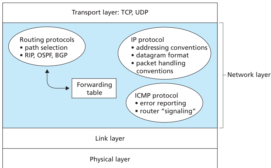
Figure 4.12 ♦ A look inside the Internet's network layer
