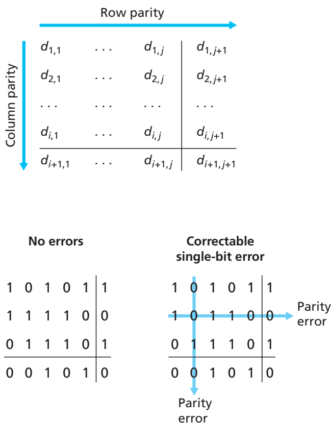
Figure 5.5 ♦ Two-dimensional even parity
