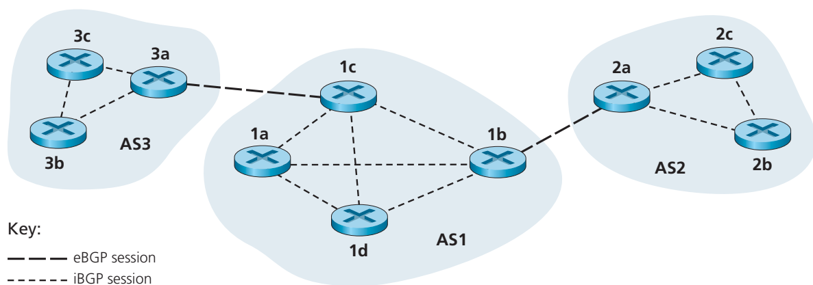
Figure 4.40 ♦ eBGP and iBGP sessions
