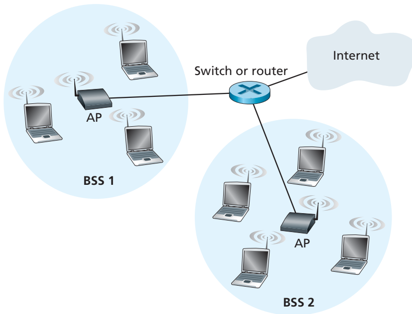
Figure 6.7 ♦ IEEE 802.11 LAN architecture
