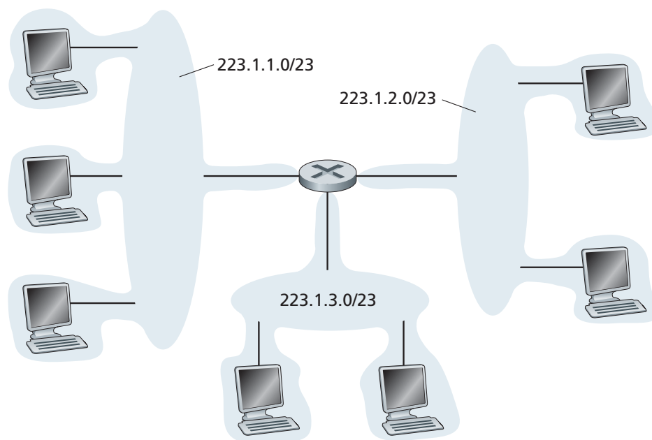
Figure 4.16 ♦ Subnet addresses
