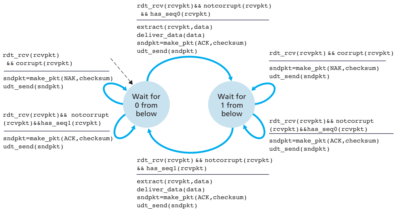
Figure 3.12 ♦ rdt2.1 receiver
