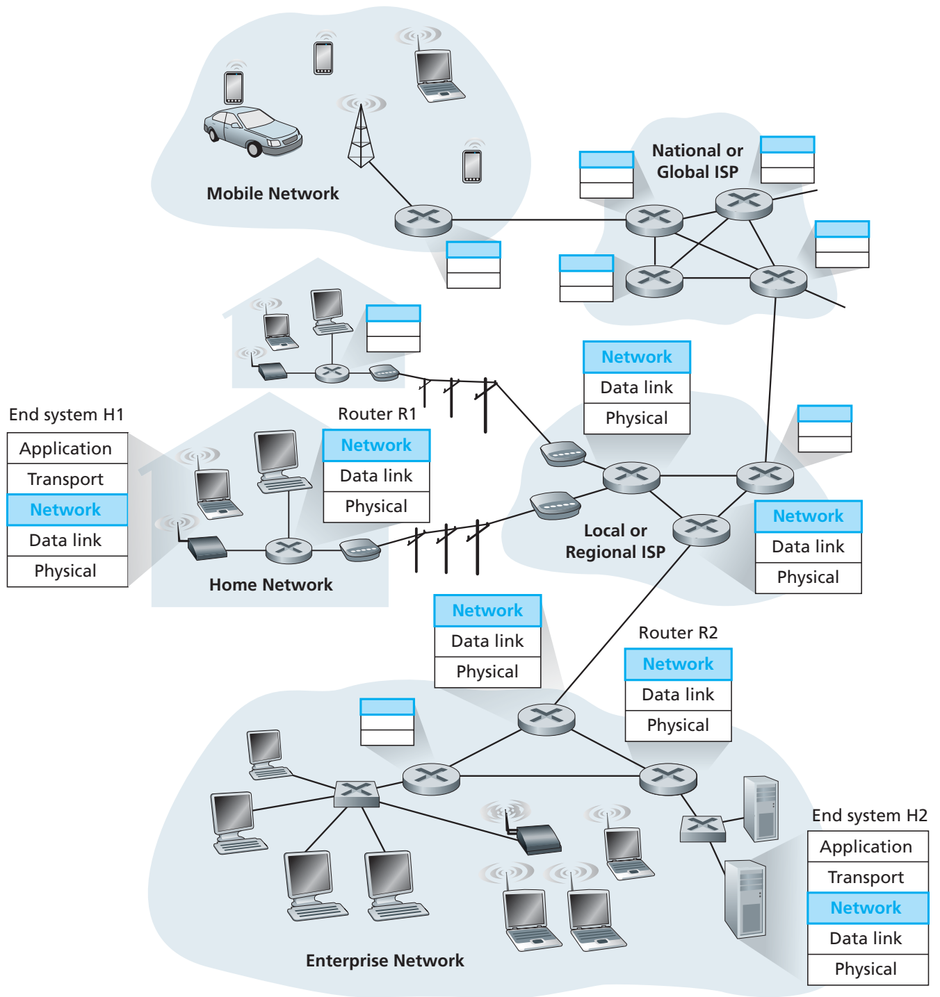
Figure 4.1 ♦ The network layer
