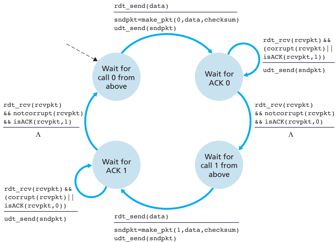
Figure 3.13 ♦ rdt2.2 sender
