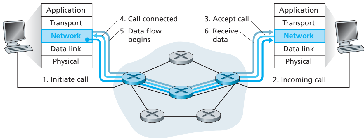
Figure 4.4 ♦ Virtual-circuit setup
