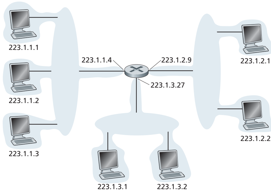
Figure 4.15 ♦ Interface addresses and subnets
