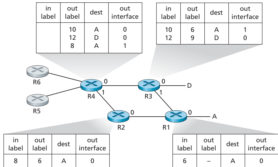
Figure 5.29 ♦ MPLS-enhanced forwarding
