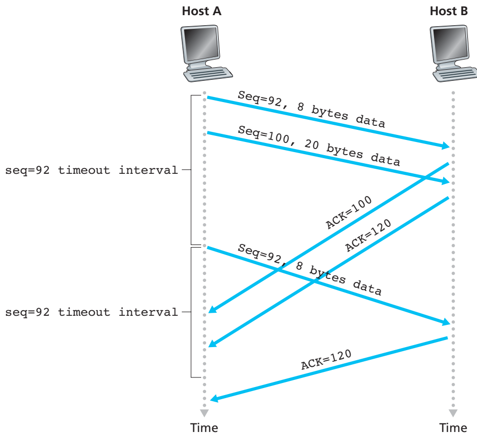
Figure 3.35 ♦ Segment 100 not retransmitted
