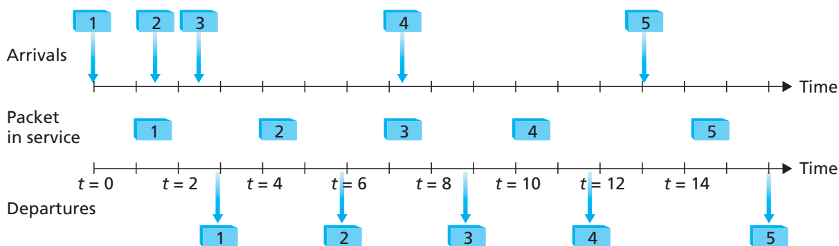
Figure 7.18 ♦ The FIFO queue in operation
