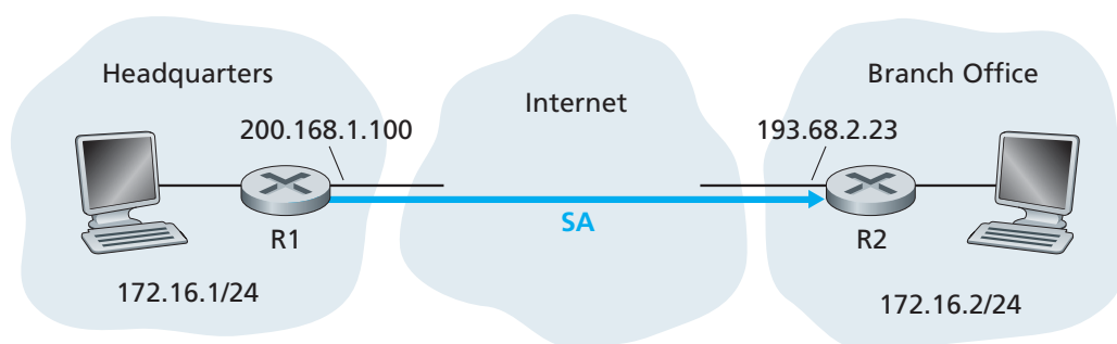
Figure 8.28 ♦ Security Association (SA) from R1 to R2
