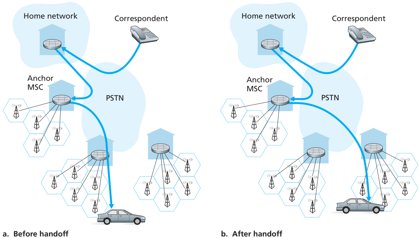
Figure 6.32 ♦ Rerouting via the anchor MSC
