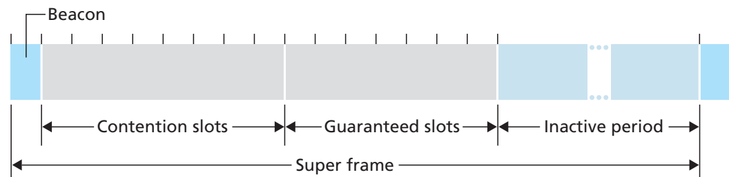
Figure 6.17 ♦ Zigbee 802.14.4 super-frame structure
