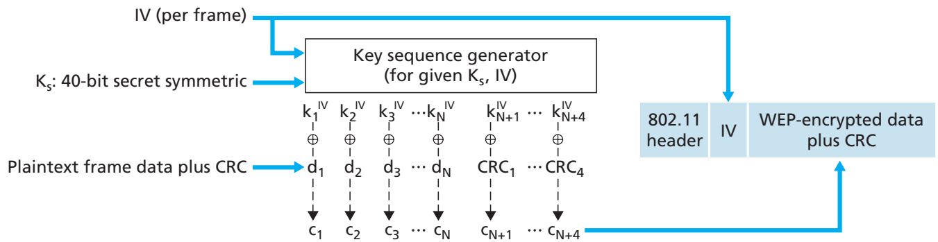
Figure 8.30 ♦ 802.11 WEP protocol
