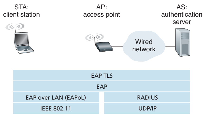
Figure 8.32 ♦ EAP is an end-to-end protocol. EAP messages are encapsulated using EAPoL over the wireless link between the client and the access point, and using RADIUS over UDP/IP between the access point and the authentication server
