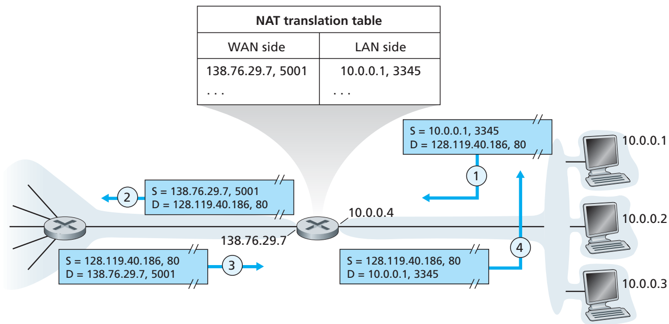
Figure 4.22 ♦ Network address translation
