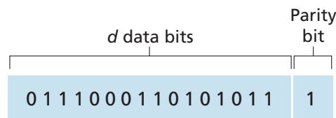
Figure 5.4 ♦ One-bit even parity
