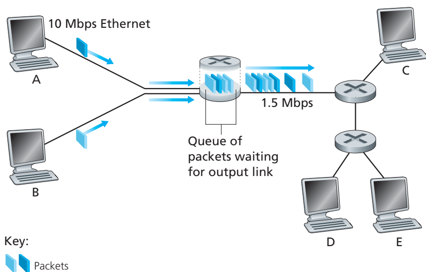
Figure 1.12 ♦ Packet switching
