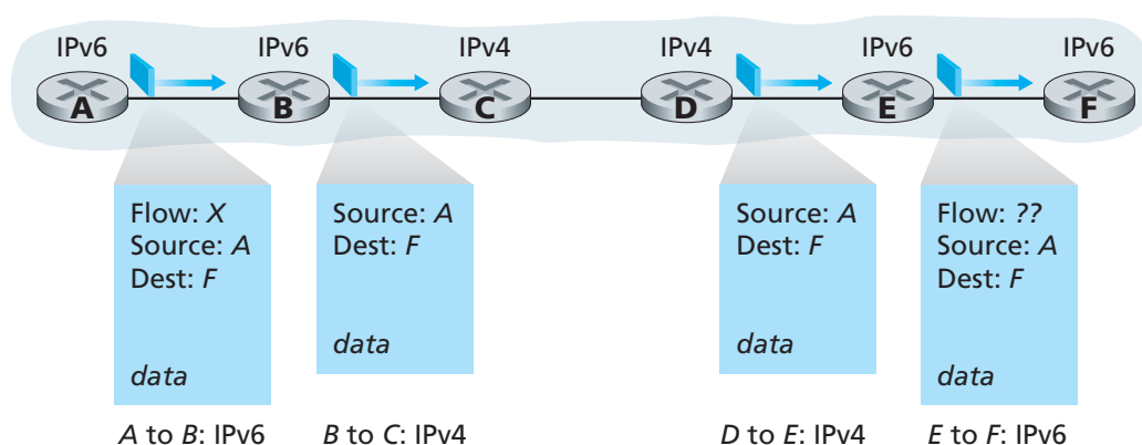
Figure 4.25 ♦ A dual-stack approach
