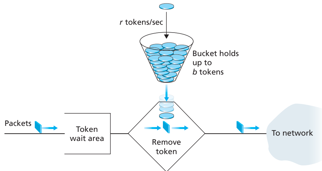
Figure 7.23 ♦ The leaky bucket policer
