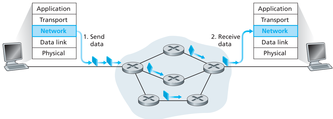
Figure 4.5 ♦ Datagram network
