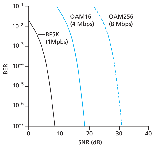
Figure 6.3 ♦ Bit error rate, transmission rate, and SNR
