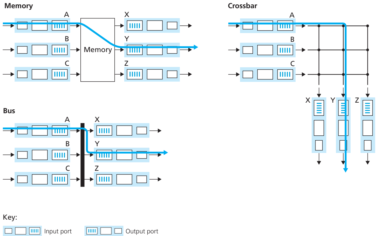
Figure 4.8 ♦ Three switching techniques
