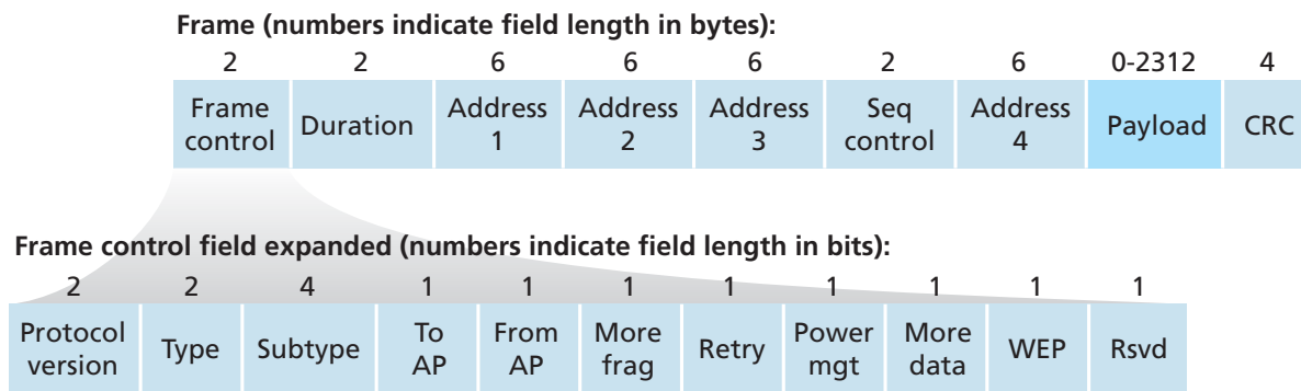
Figure 6.13 ♦ The 802.11 frame
