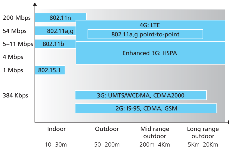
Figure 6.2 ♦ Link characteristics of selected wireless network standards
