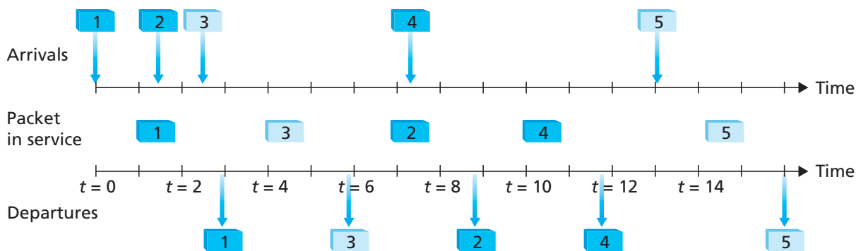
Figure 7.21 ♦ Operation of the two-class round robin queue
