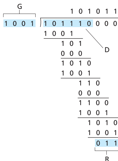
Figure 5.7 ♦ A sample CRC calculation
