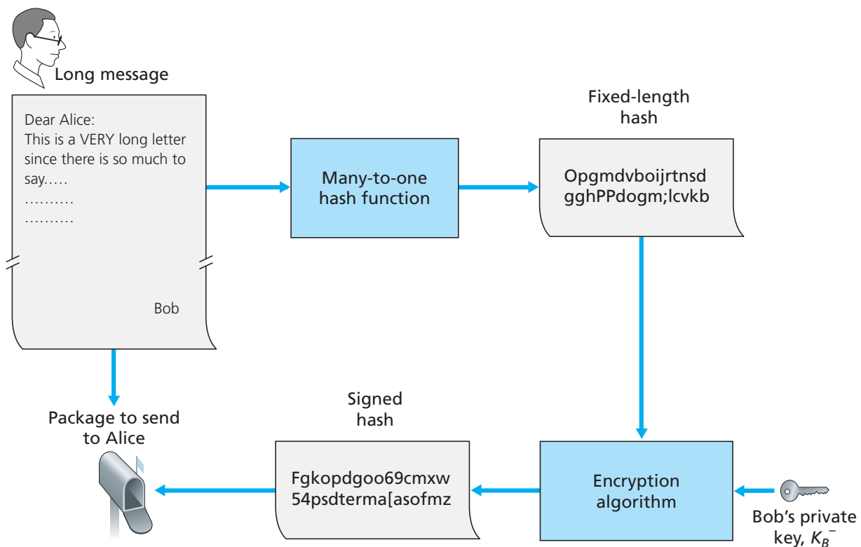
Figure 8.11 ♦ Sending a digitally signed message
