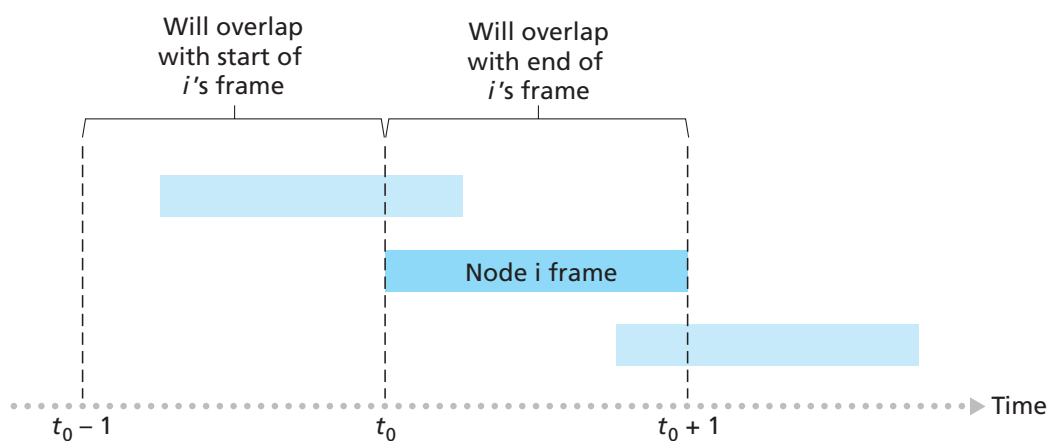
Figure 5.11 ♦ Interfering transmissions in pure ALOHA
