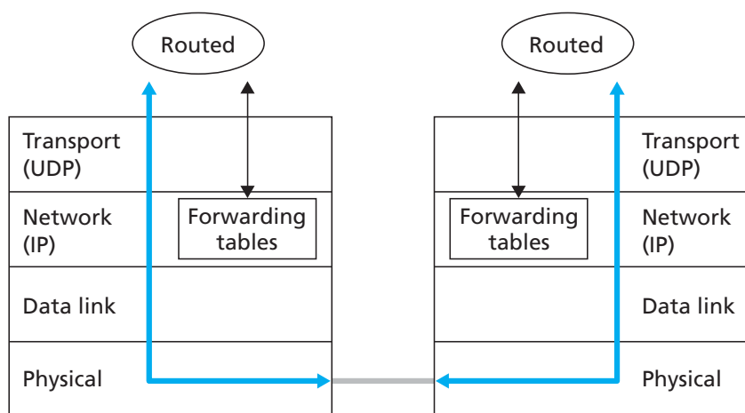
Figure 4.39 ♦ Implementation of RIP as the routed daemon
