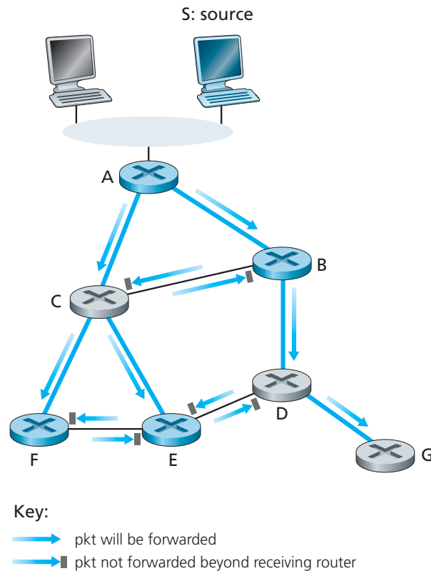
Figure 4.50 ♦ Reverse path forwarding, the multicast case
