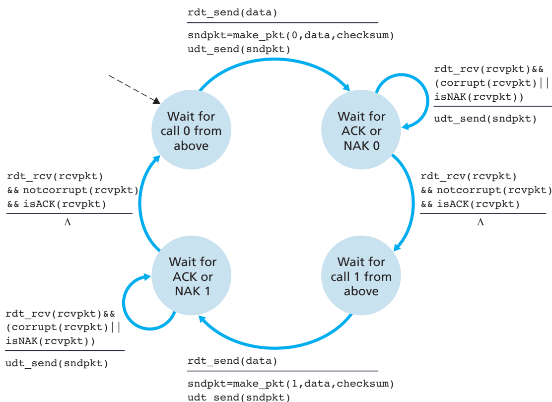
Figure 3.11 ♦ rdt2.1 sender
