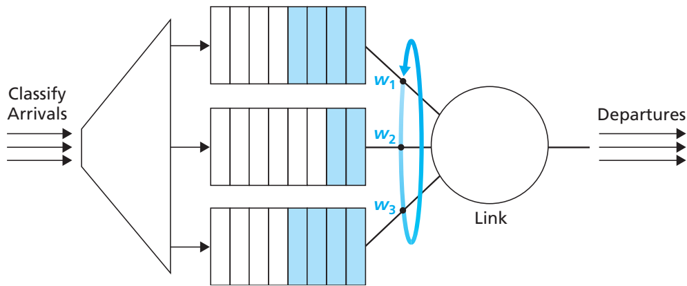
Figure 7.22 ♦ Weighted fair queuing (WFQ)
