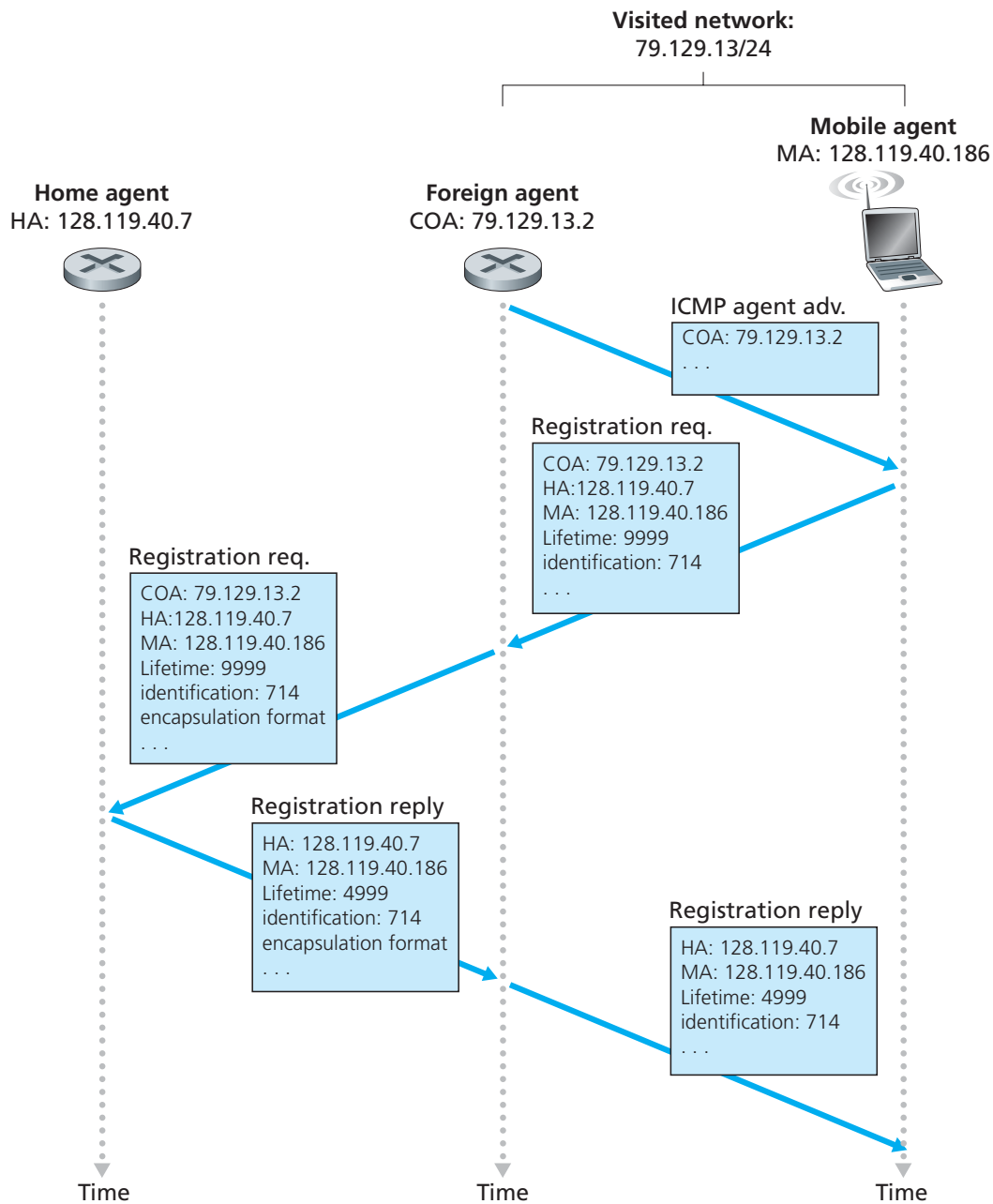
Figure 6.28 ♦ Agent advertisement and mobile IP registration
