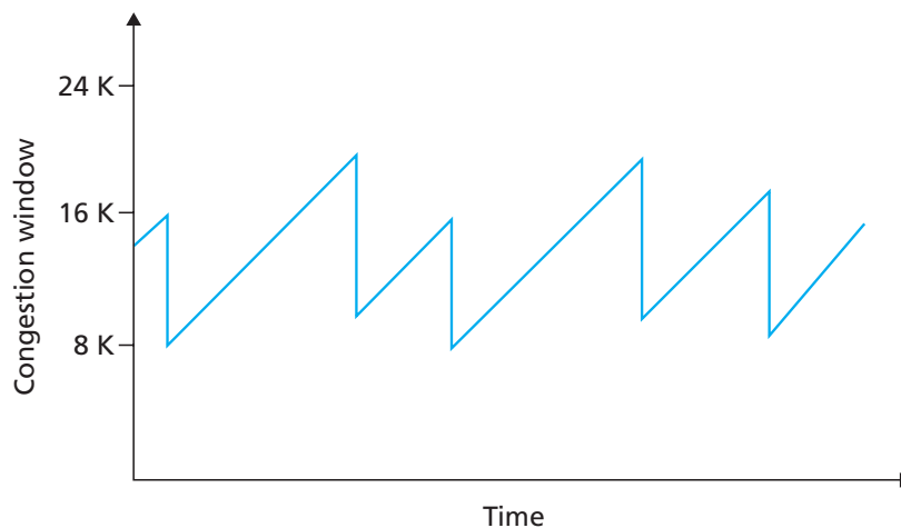
Figure 3.54 ♦ Additive-increase, multiplicative-decrease congestion control
