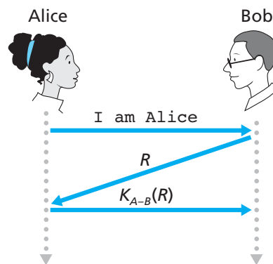
Figure 8.18 ♦ Protocol ap4.0 and a failure scenario
