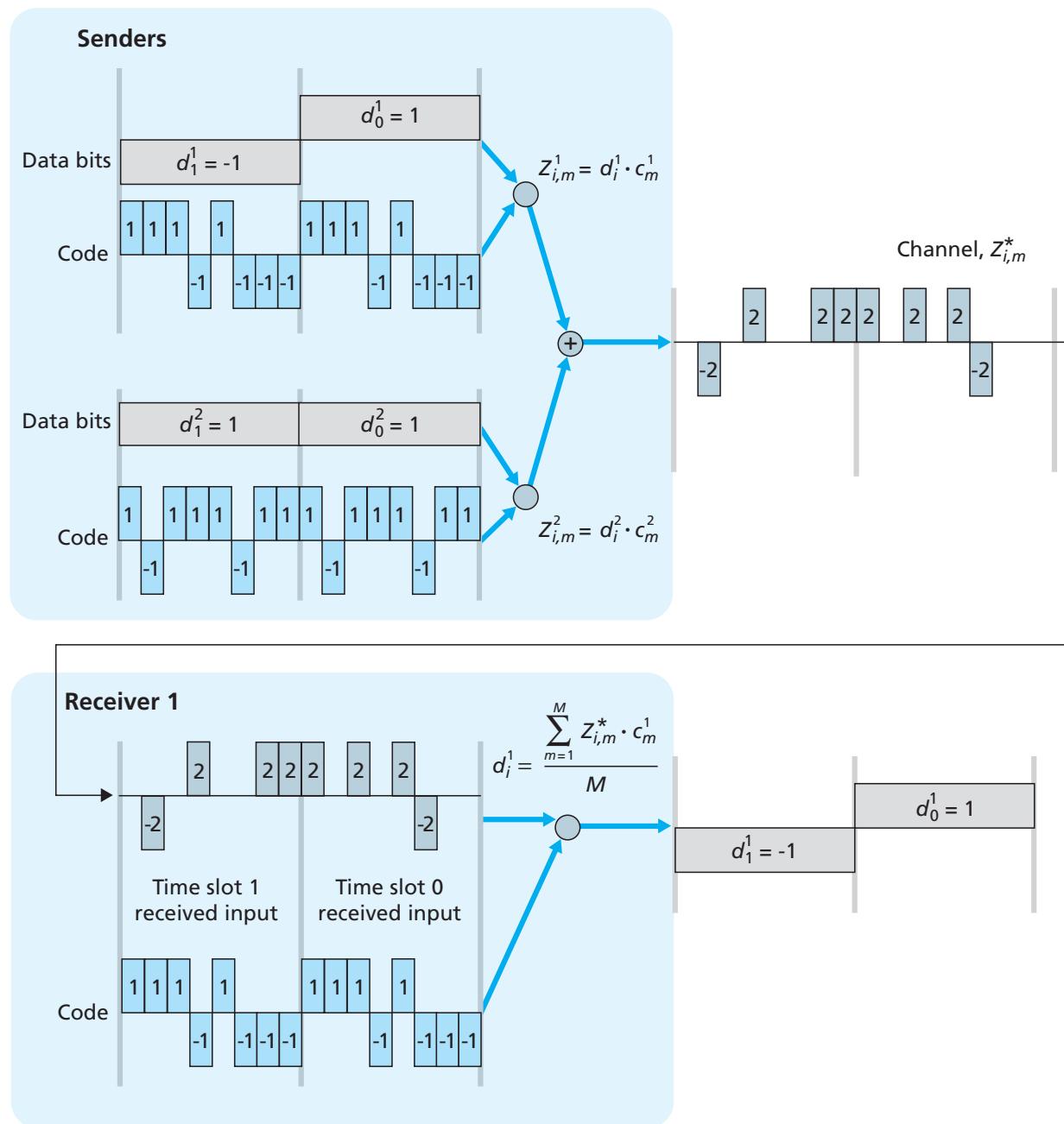
Figure 6.6 ♦ A two-sender CDMA example
