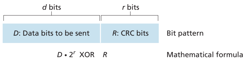
Figure 5.6 ♦ CRC
