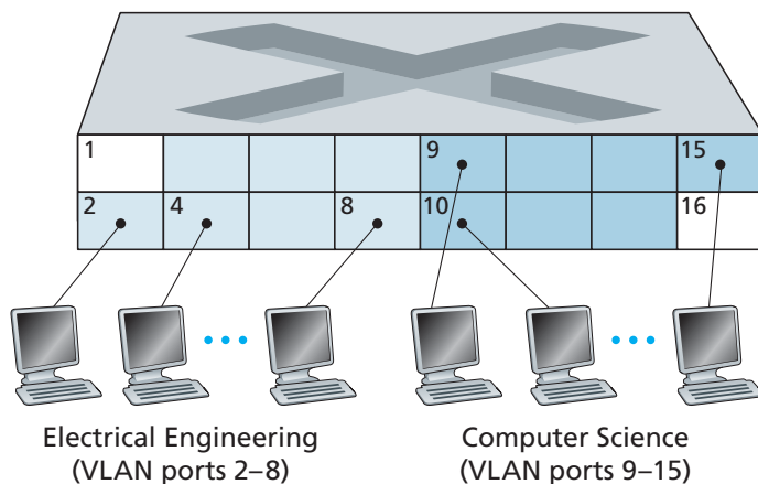
Figure 5.25 ♦ A single switch with two configured VLANs
